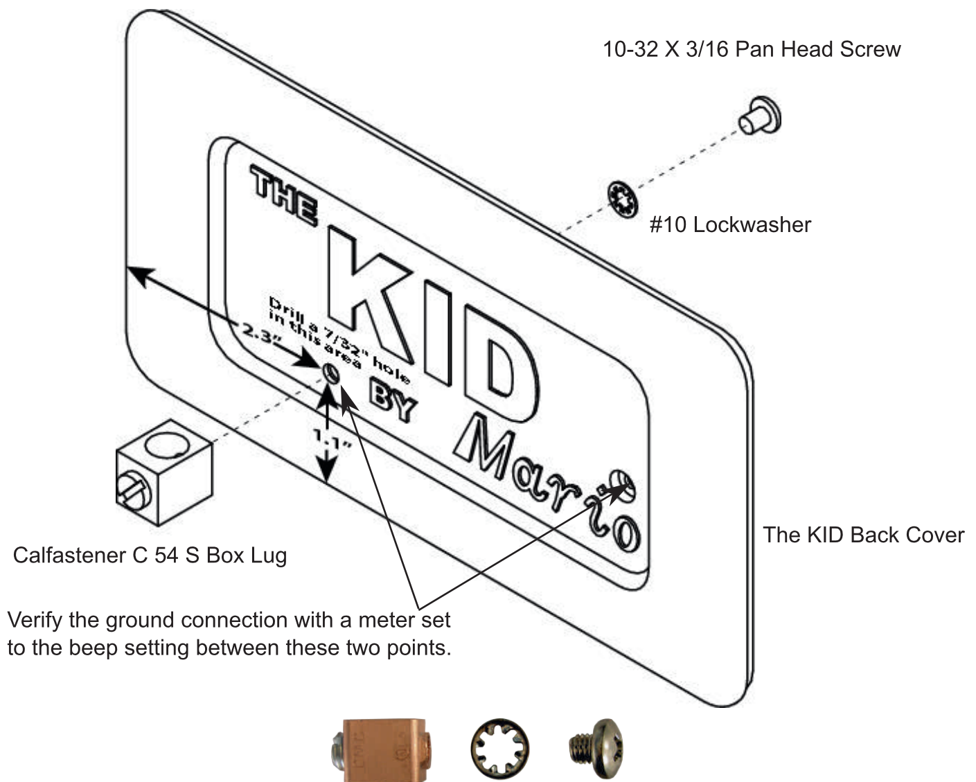
Grounding Lug hardware supplied with The Kid
